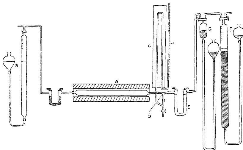
Fig. 1. Static system
